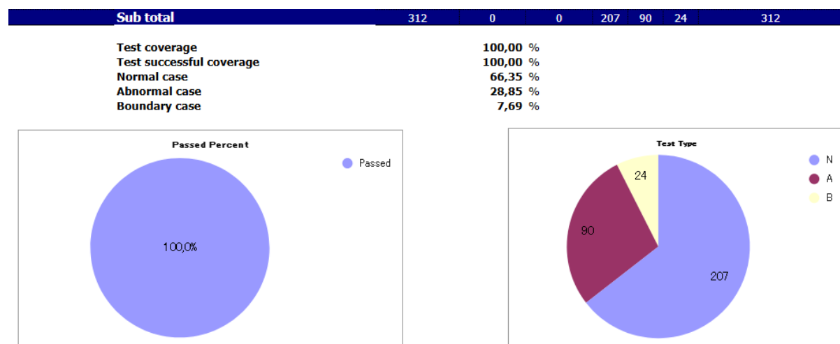
Figure 5.1: Unit test report
